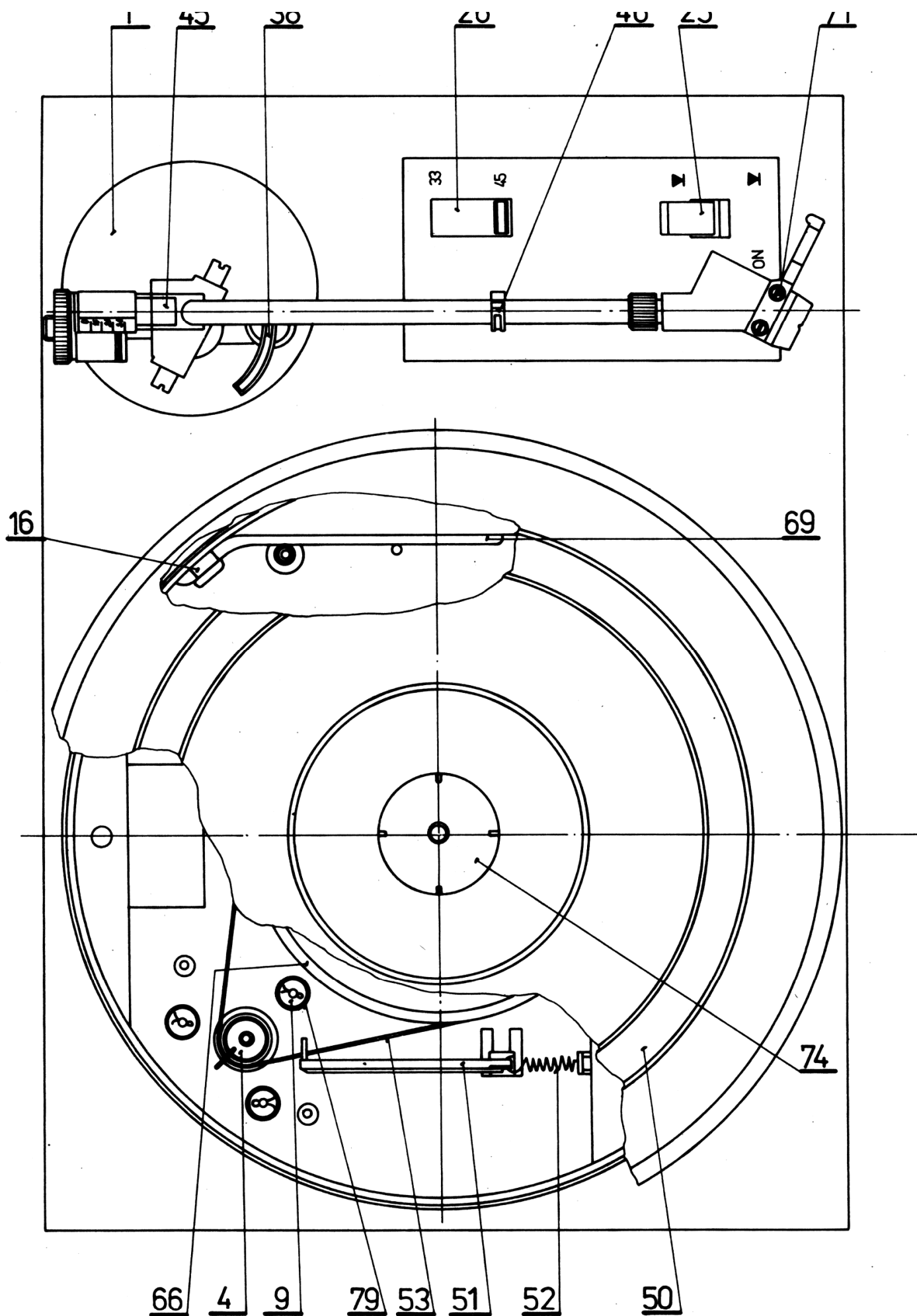
Obr. 4. Chassis HC 30 - pohled shora
